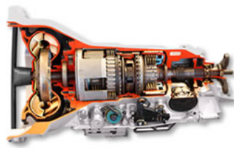
Transmission/Transfer Case
